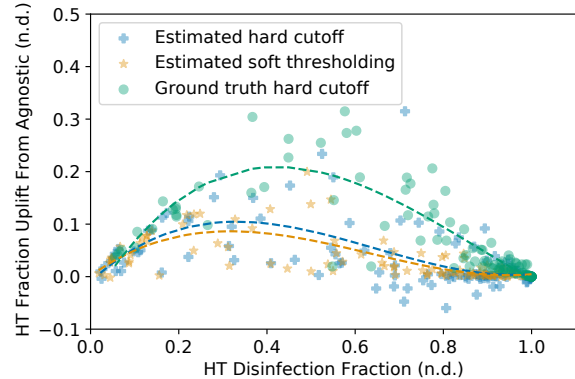
Fig. 4: Increase in disinfected high-touch surface fraction over surface agnostic planning for different surface-aware disinfection strategies over 10 ScanNet Scenes (Best seen in color)
